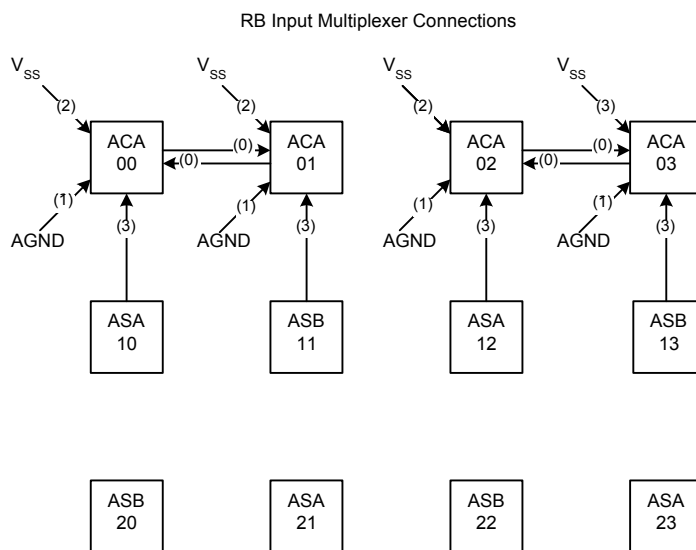
Figure 20: RBotMux Connections
