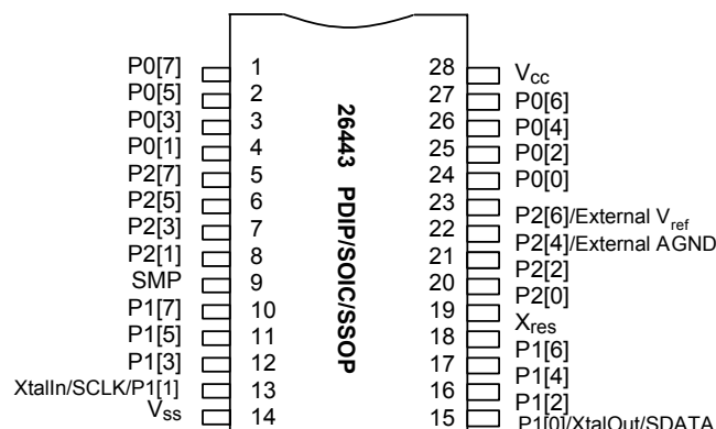
Figure 4: 26443 PDIP/SOIC/SSOP
