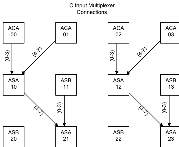
Figure 24: CMux Connections
