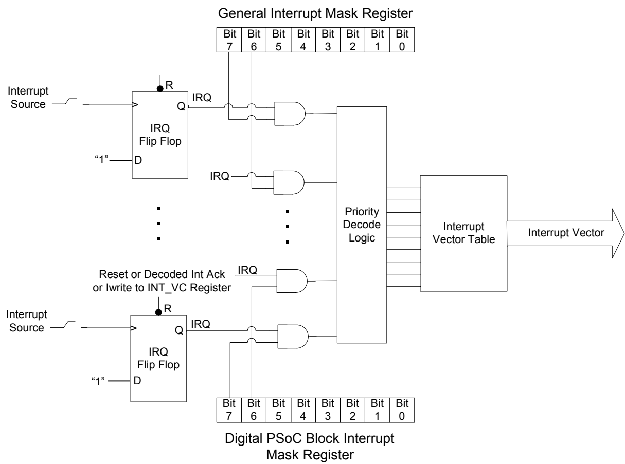
Figure 10: Interrupts Overview
